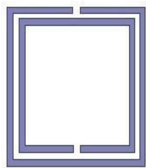
Figure 4 Defected Ground Structure
