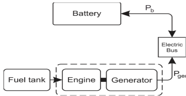
Figure 2: Schematic diagram of a HEV
