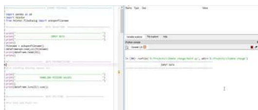
Fig. 1 Editor Window
